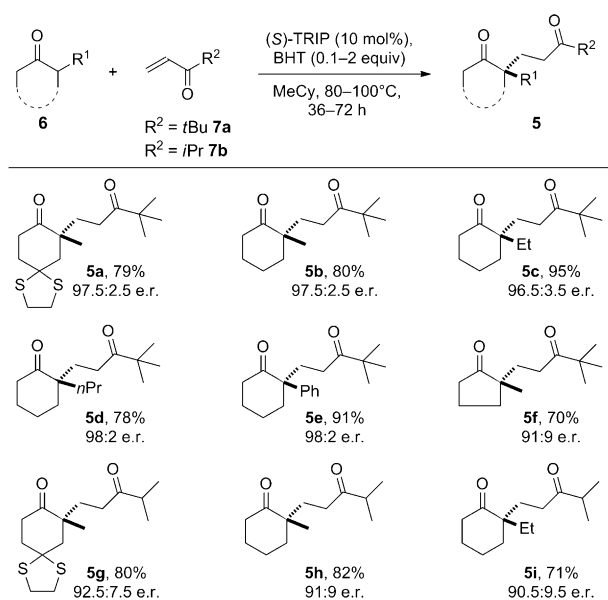
Scheme 3. Substrate scope of the enantioselective Michael reaction.
