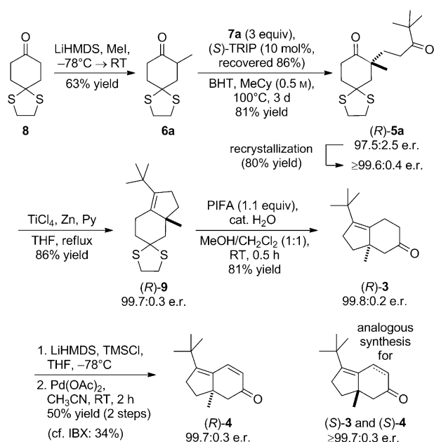
Scheme 4. Synthesis of the target odorants 3 and 4 in both enantiomeric forms with high enantiomeric purity ( \geq 99.7:0.3 e.r.). LiHMDS = lithium bis(trimethylsilyl)amide, py = pyridine, PIFA = phenyliodine bis(trifluoroacetate).
